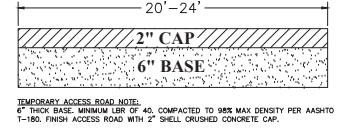
Stabilized Access/ Maintenance Drive
