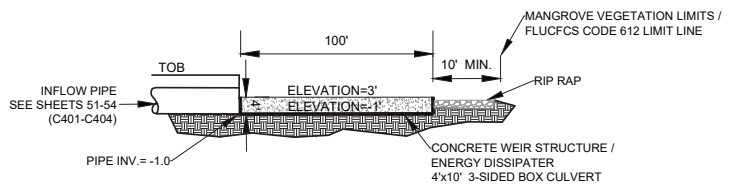
Longitudinal Cross Section of Dissipater
