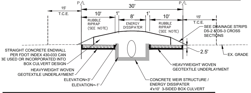
Drainage Strip Cross Section of Dissipater
