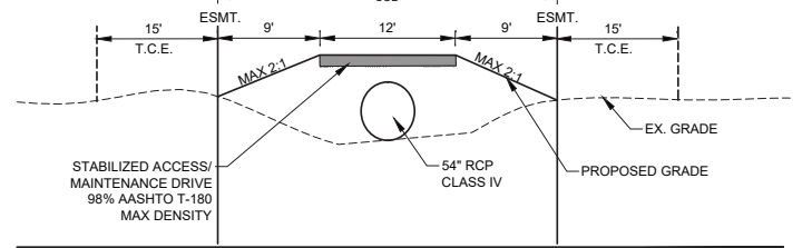
Drainage Strip (DS-3) Cross Section Prior to Dissipater
